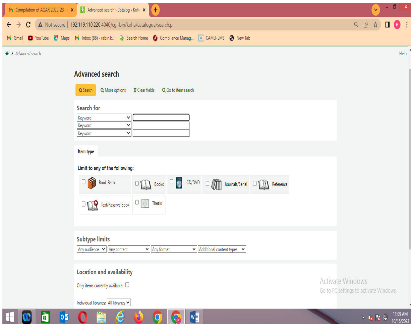
Fig 8: OPAC Page
