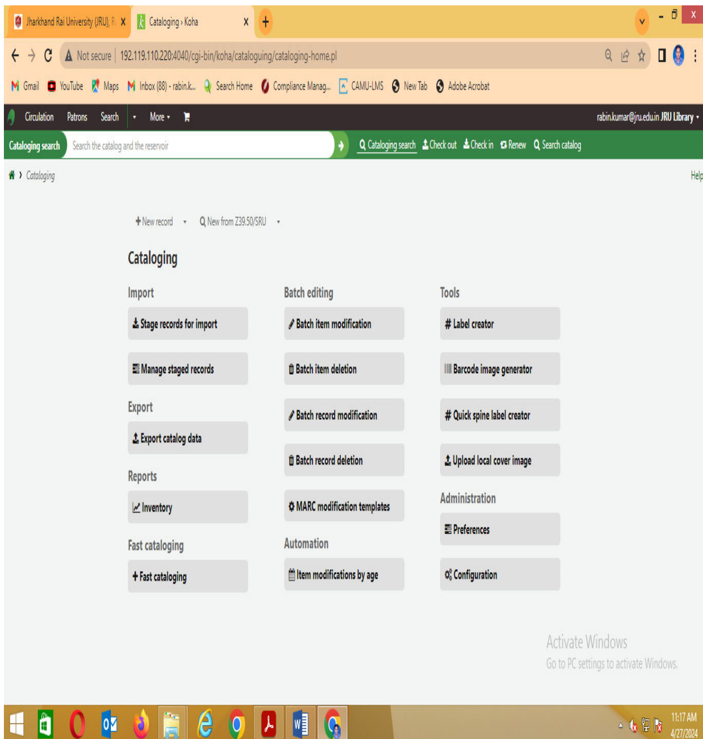
Fig4: Catalogue page
